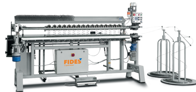
FA-20 Assembly machine for Bonnell spring units
